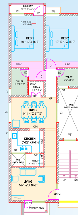
Flat : C 2, D 2 - First Floor
