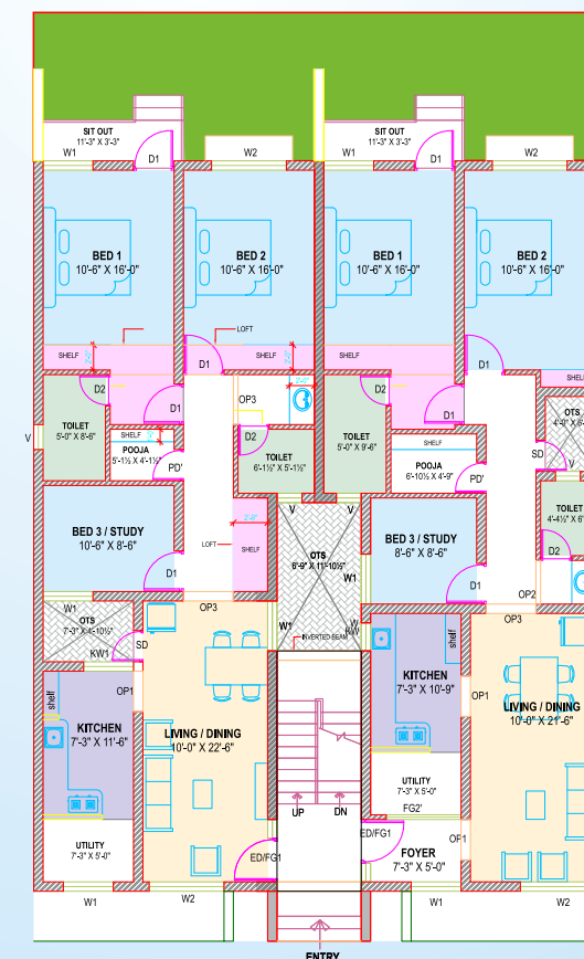
Flat : E 1, G 1, I 1 - F 1, H 1, J 1 Ground Floor
